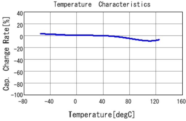
■ GCM155R72A102KA37 C-Temp. capchange, DCO. 0V, AC1. 0Vrm
