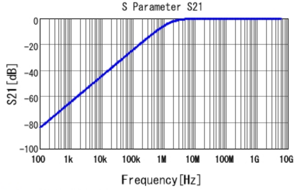
■ GCM155R72A102KA37 S21 DCOV, 25degC
