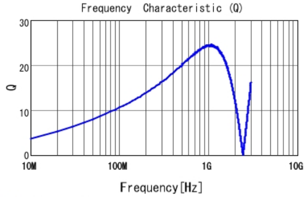
■ LQG15HN22NJ02 Q
