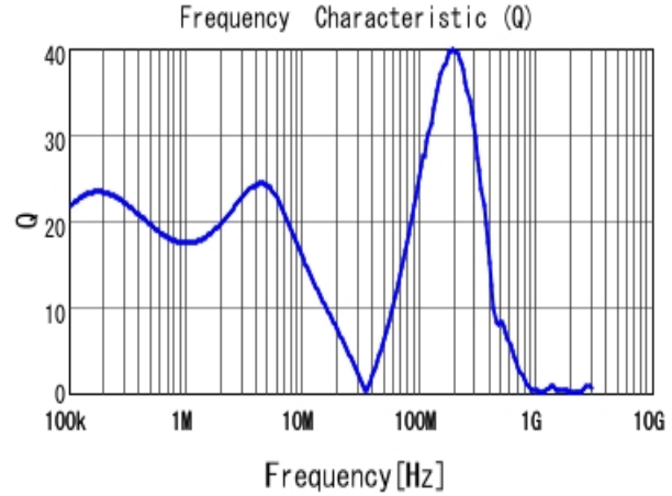
■ LQH5BPH100MT0 Q
