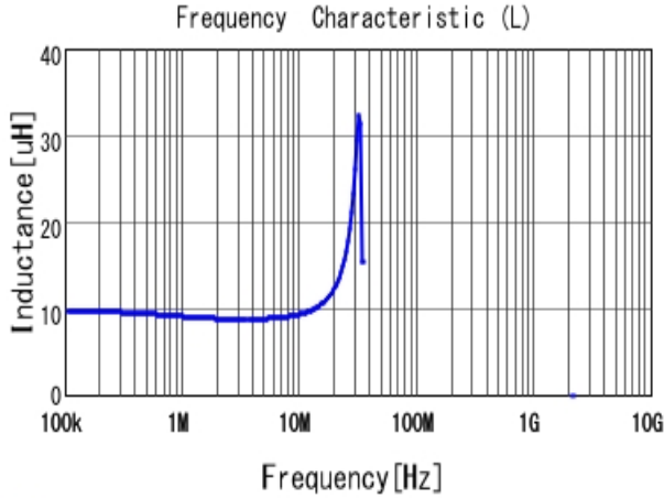
■ LQH5BPH100MT0 L
