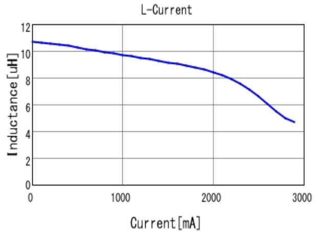
■ LQH5BPH100MT0 L-Current 20degC
