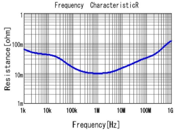
■ ECASD41A336M025K00 R DC0V, 25degC
