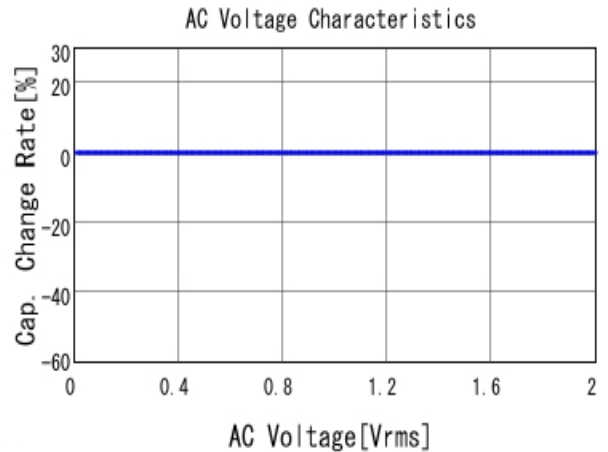
■ ECASD41A336M025K00 C-AC Voltage capchange, DC0V, 25.0
