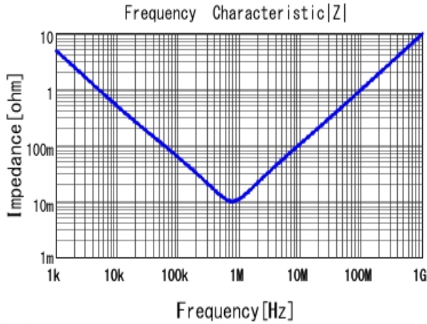
■ ECASD41A336M025K00 |Z| DC0V, 25degC
