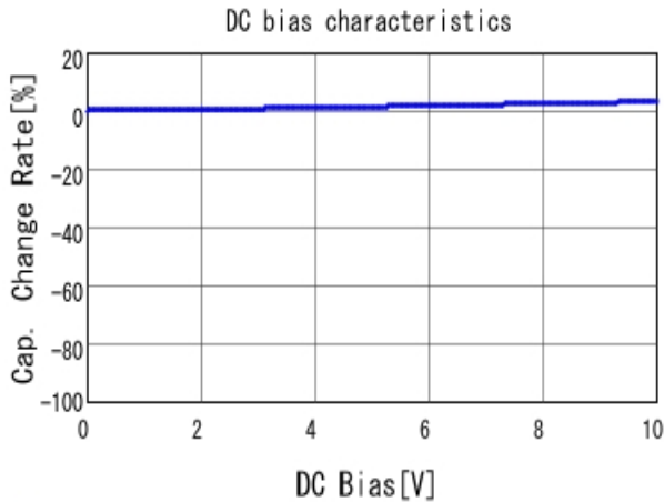
■ ECASD41A336M025K00 C-DC bias capchange, 25.0degC, AC1
