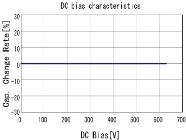
■ KCA55L7UMF102KL01 C-DC bias capchange, 25.0degC, AC1V
