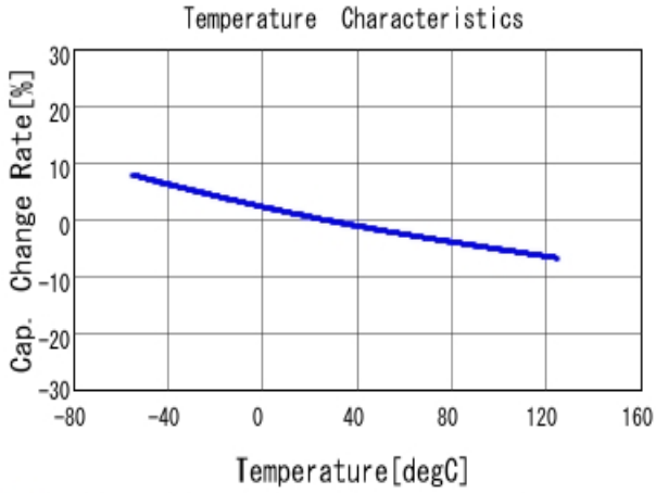
■ KCA55L7UMF102KL01 C-Temp. capchange, DCOV, AC1Vrms
