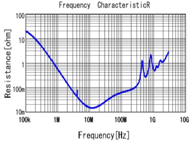
■ KCA55L7UMF102KL01 R DC0V, 25degC
