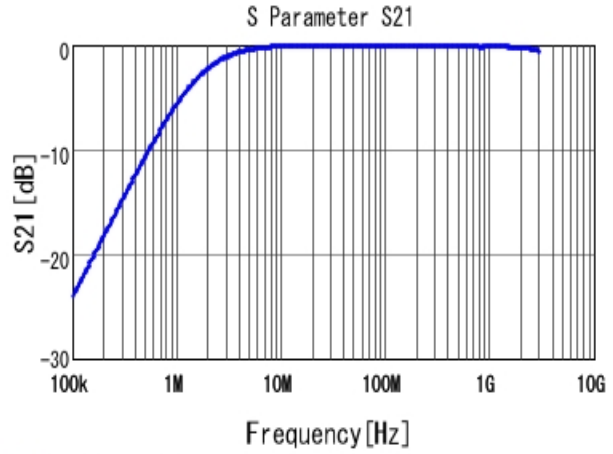
■ KCA55L7UMF102KL01 S21 DCOV, 25degC
