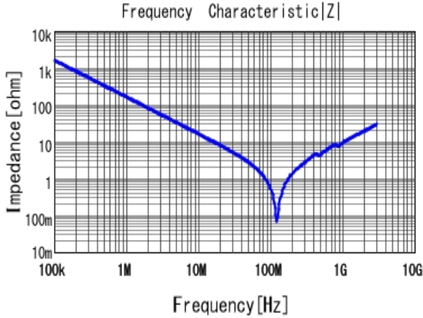
■ KCA55L7UMF102KL01 |Z| DC0V, 25degC
