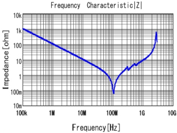
■ KCA55L7UMF152KL01 |Z| DC0V, 25degC
