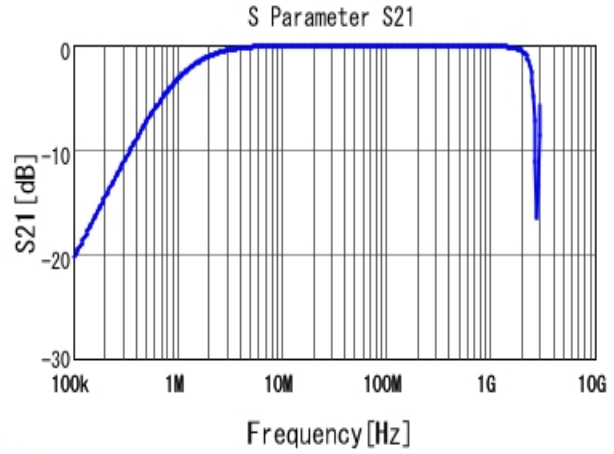
■ KCA55L7UMF152KL01 S21 DCOV, 25degC
