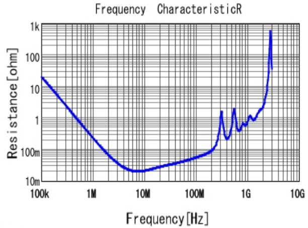
■ KCA55L7UMF152KL01 R DC0V, 25degC
