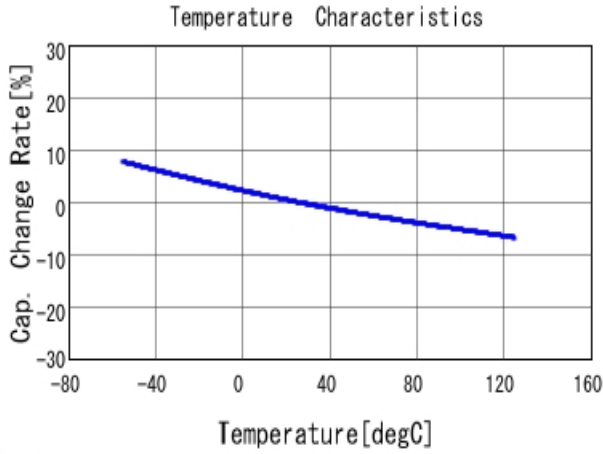
■ KCA55L7UMF152KL01 C-Temp. capchange, DCOV, AC1Vrms
