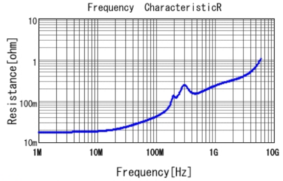
■ GRM1857U1A822JA44 R DCOV, 25degC
