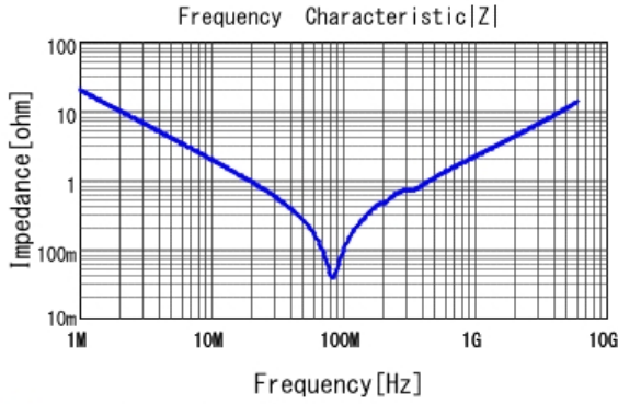
■ GRM1857U1A822JA44 |Z| DCOV, 25degC
