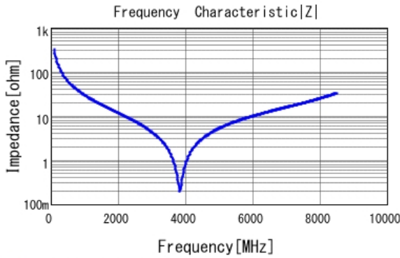
■ GJM1555C1H5R0CB01 |Z| DCOV, 25degC
