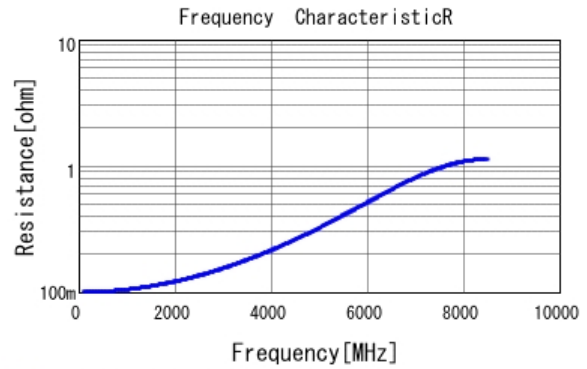
■ GJM1555C1H5R0CB01 R DCOV, 25degC
