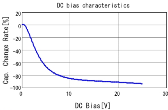
■ GRM155R61E105MA12 C-DC bias capchange, 25.0degC, AC1.
