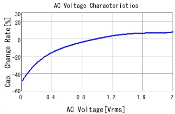
■ GRM155R61E105MA12 C-AC Voltage capchange, DCOV, 25.0d
