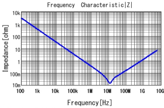
■ GRM155R61E105MA12 |Z| DCOV, 25degC
