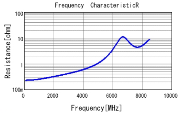
■ GCM1555C1H6R8BA16 R DCOV, 25degC
