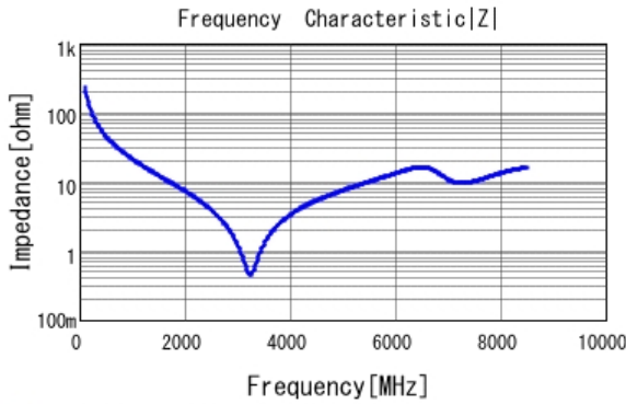
■ GCM1555C1H6R8BA16 |Z| DCOV, 25degC
