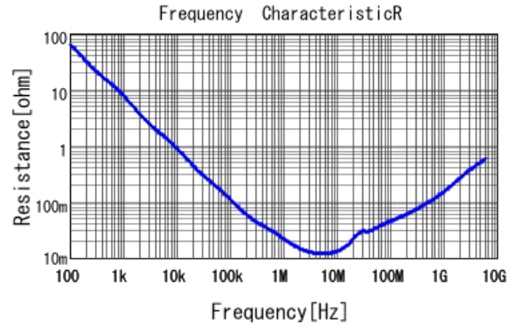
■ GRM155C81A105KA12 R DC0V, 25degC
