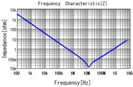
■ GRM155C81A105KA12 |Z| DC0V, 25degC
