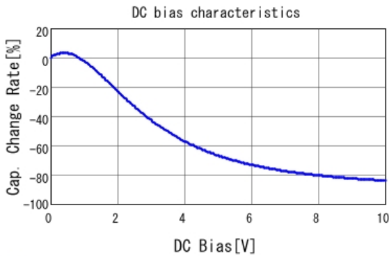
■ GRM155C81A105KA12 C-DC bias capchange, 25.0degC, AC1.
