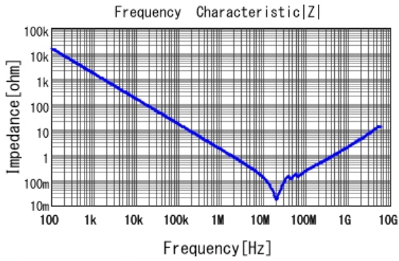
■ GCD21BR72A104KA01 |Z| DC0V, 25degC
