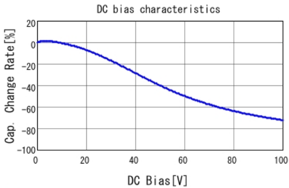
■ GCD21BR72A104KA01 C-DC bias capchange, 25.0degC, AC1.
