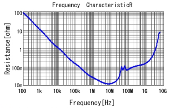
■ GCD21BR72A104KA01 R DC0V, 25degC
