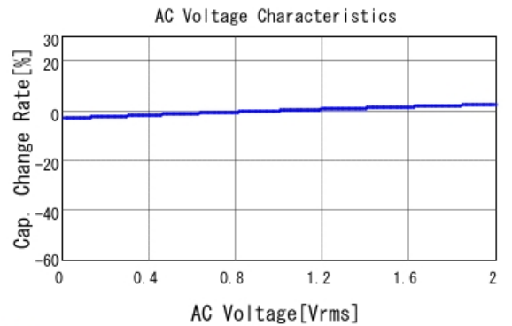
■ GCD21BR72A104KA01 C-AC Voltage capchange, DC0V, 25.0d
