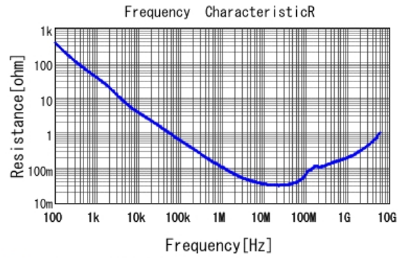
■ GRM155R71H223KA12 R DCOV, 25degC
