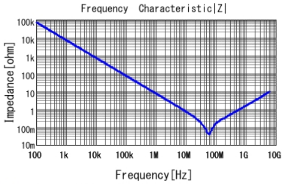
■ GRM155R71H223KA12 |Z| DCOV, 25degC
