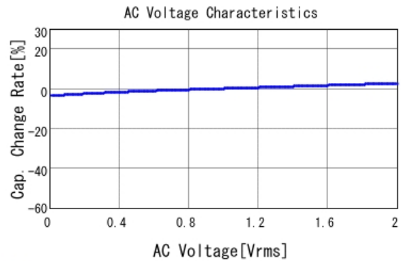
■ GRM155R71H223KA12 C-AC Voltage capchange, DCOV, 25.0d
