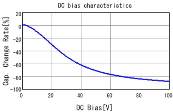
■ GCJ21BC72A105KE02 C-DC bias capchange, 25.0degC, AC1.
