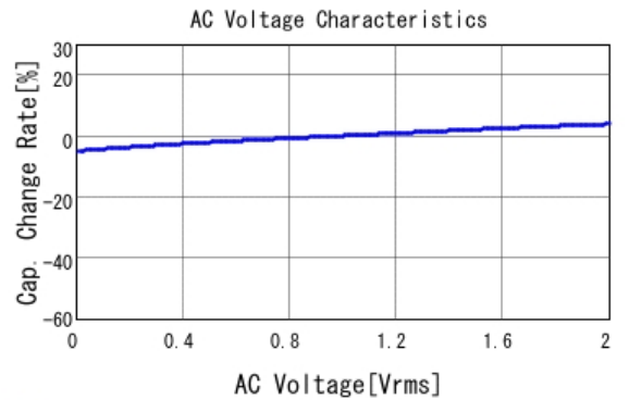
■ GCJ21BC72A105KE02 C-AC Voltage capchange, DC0V, 25.0d
