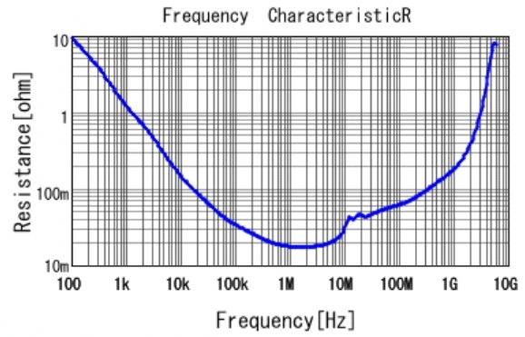
■ GCJ21BC72A105KE02 R DC0V, 25degC
