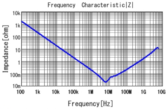
■ GCJ21BC72A105KE02 |Z| DC0V, 25degC
