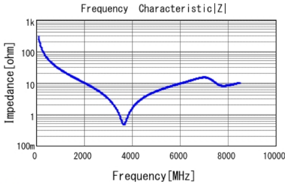
■ GCM1555C1H5R6BA16 |Z| DC0V, 25degC
