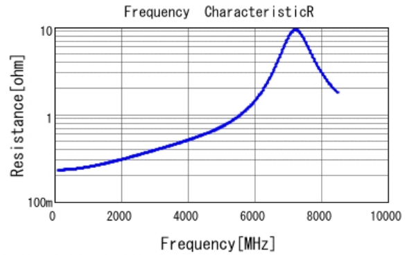
■ GCM1555C1H5R6BA16 R DC0V, 25degC
