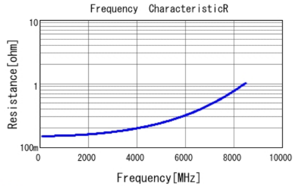
■ GJM1555C1H2R4CB01 R DC0V, 25degC
