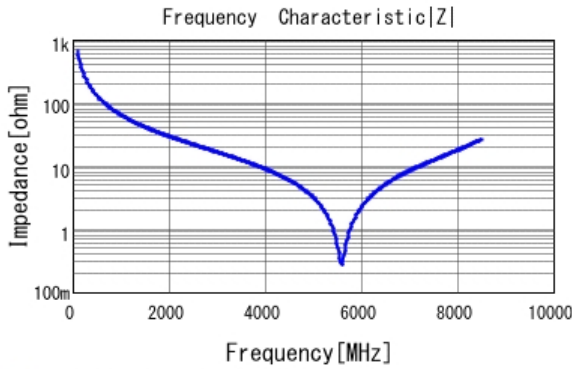
■ GJM1555C1H2R4CB01 |Z| DC0V, 25degC
