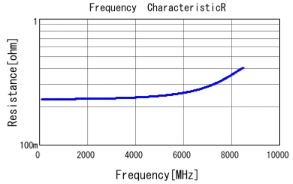
■ GJM1555C1H1R3CB01 R DCOV, 25degC
