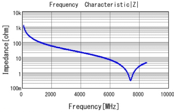
■ GJM1555C1H1R3CB01 |Z| DCOV, 25degC
