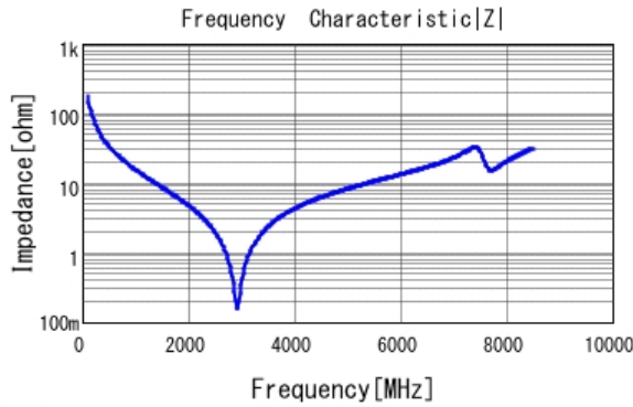
■ GJM1555C1H9R1FB01 |Z| DCOV, 25degC
