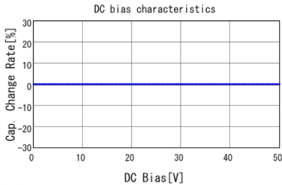
■ GJM1555C1H9R1FB01 C-DC bias capchange, 25.0degC, AC1V
