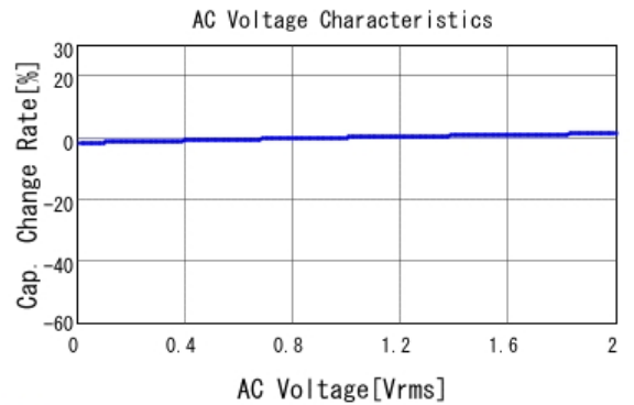
■ GCD188R72A102KA01 C-AC Voltage capchange, DCOV, 25.0d
