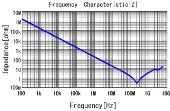
■ GCD188R72A102KA01 |Z| DCOV, 25degC
