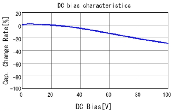
■ GCD188R72A102KA01 C-DC bias capchange, 25.0degC, AC1.
