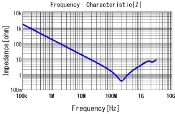
■ GCJ21AR72E102KXJ1 |Z| DCOV, 25degC
