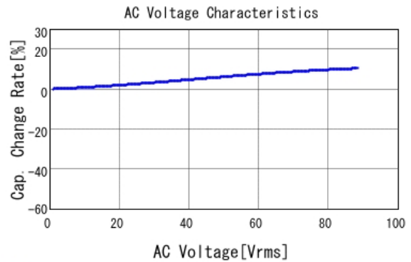
■ GCJ21AR72E102KXJ1 C-AC Voltage capchange, DCOV, 25.0d
