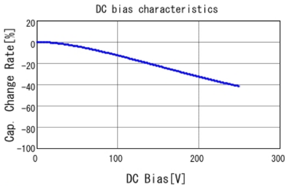
■ GCJ21AR72E102KXJ1 C-DC bias capchange, 25.0degC, AC1V
