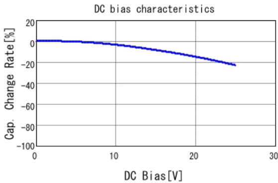
■ GCD188R71E473KA01 C-DC bias capchange, 25.0degC, AC1.
