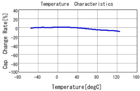
■ GCD188R71E473KA01 C-Temp. capchange, DC0.0V, AC1.0Vrm
