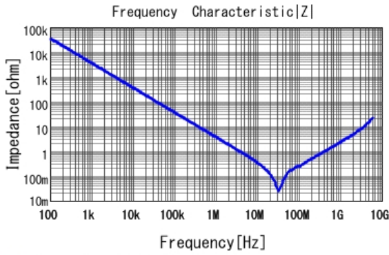
■ GCD188R71E473KA01 |Z| DCOV, 25degC
