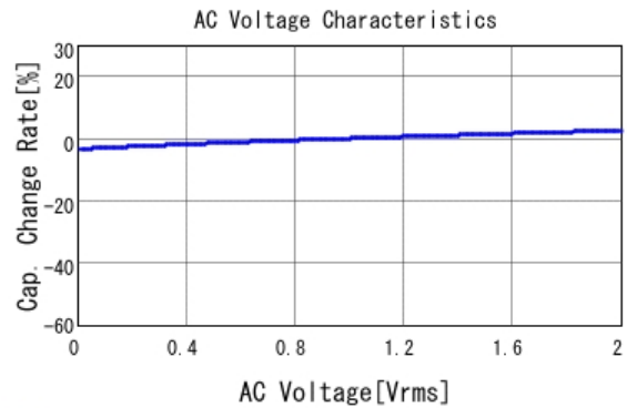
■ GCD188R71E473KA01 C-AC Voltage capchange, DCOV, 25.0d
