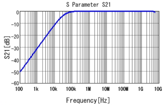
■ GCD188R71E473KA01 S21 DC0V, 25degC
