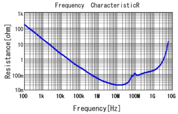
■ GCD188R71E473KA01 R DCOV, 25degC
