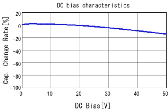
GCD188R71H472KA01 C-DC bias capchange, 25.0degC, AC1.
