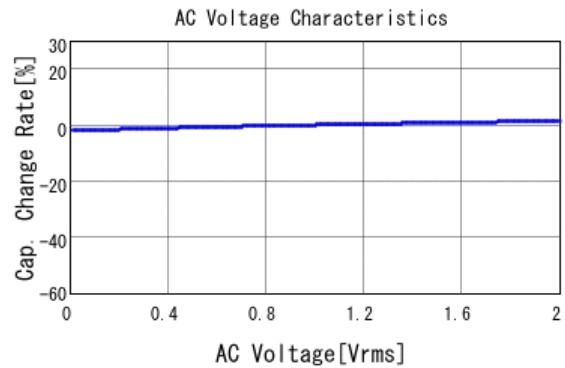
GCD188R71H472KA01 C-AC Voltage capchange, DCOV, 25.0d
