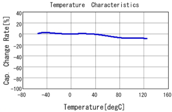
■ GCD188R71H472KA01 C-Temp. capchange, DC0.0V, AC1.0Vrm
