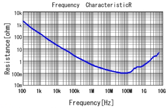
GCD188R71H472KA01 R DCOV, 25degC
