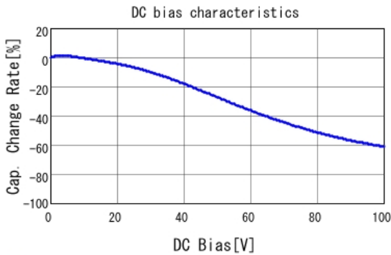
■ GCJ219R72A333KA01 C-DC bias capchange, 25.0degC, AC1.
