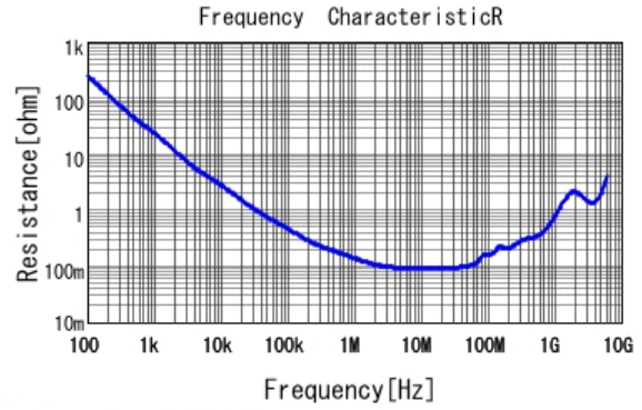
■ GCJ219R72A333KA01 R DCOV, 25degC
