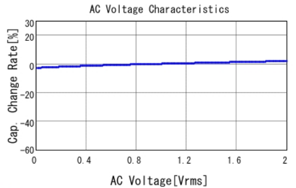
■ GCJ219R72A333KA01 C-AC Voltage capchange, DCOV, 25.0d
