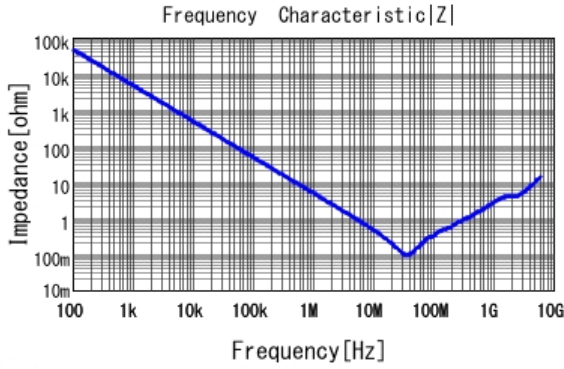
■ GCJ219R72A333KA01 |Z| DCOV, 25degC
