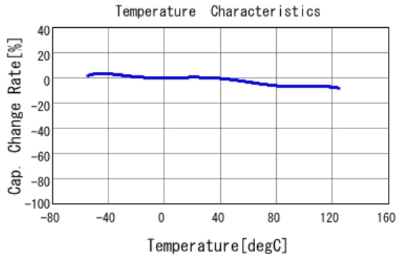
■ GCJ219R72A333KA01 C-Temp. capchange, DC0.0V, AC1.0Vrm
