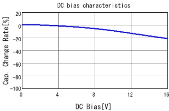
GCM188L81C224KA37 C-DC bias capchange, 25.0degC, AC1.
