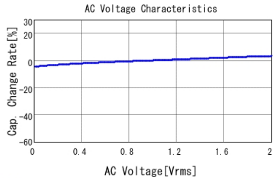
GCM188L81C224KA37 C-AC Voltage capchange, DCOV, 25.0d
