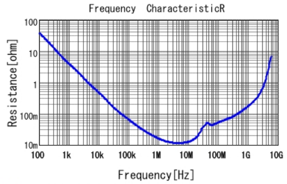
GCM188L81C224KA37 R DCOV, 25degC
