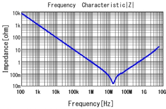
GCM188L81C224KA37 |Z| DCOV, 25degC
