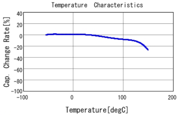
GCM188L81C224KA37 C-Temp. capchange, DC0.0V, AC1.0Vrm
