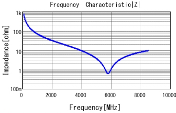
■ GCM1555C1H2R2CA16 |Z| DCOV, 25degC
