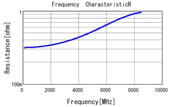
■ GCM1555C1H2R2CA16 R DCOV, 25degC
