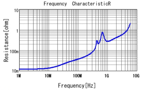
■ GCM1885C2A122JA16 R DCOV, 25degC
