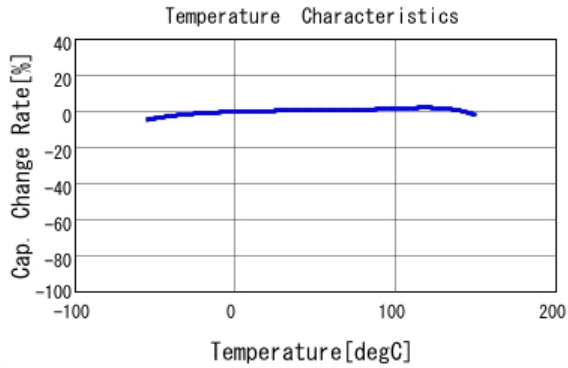
■ GCJ188R92A333KA01 C-Temp. capchange, DC0.0V, AC1.0Vrm
