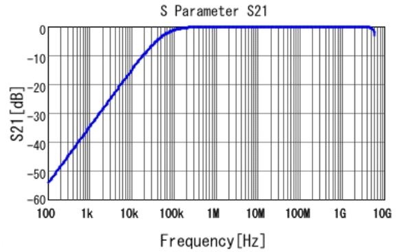
■ GCJ188R92A333KA01 S21 DC0V, 25degC
