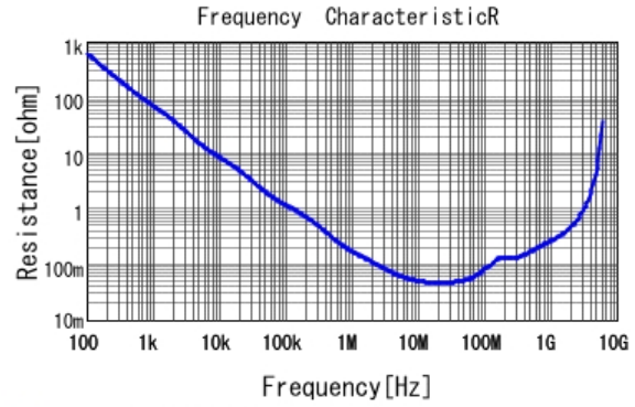
■ GCJ188R92A333KA01 R DCOV, 25degC
