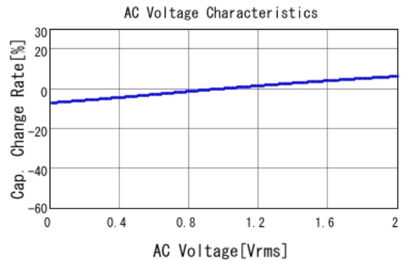
■ GCJ188R92A333KA01 C-AC Voltage capchange, DCOV, 25.0d
