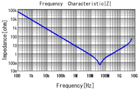
■ GCJ188R92A333KA01 |Z| DCOV, 25degC
