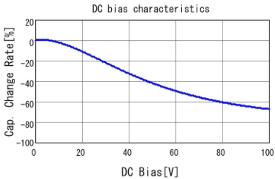
■ GCJ188R92A333KA01 C-DC bias capchange, 25.0degC, AC1.
