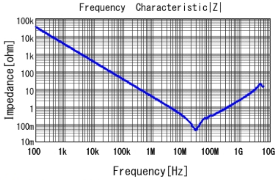
■ GCE21BR71H473KA01 |Z| DCOV, 25degC
