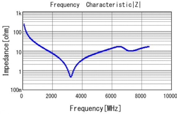
■ GCM1555C1H6R8DA16 |Z| DCOV, 25degC
