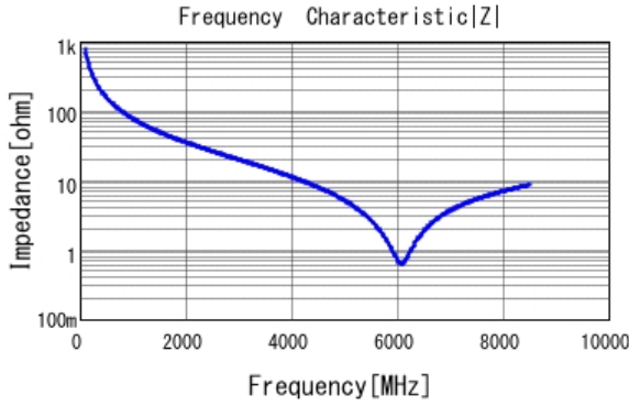
■ GCM1555C1H2R0CA16 |Z| DCOV, 25degC
