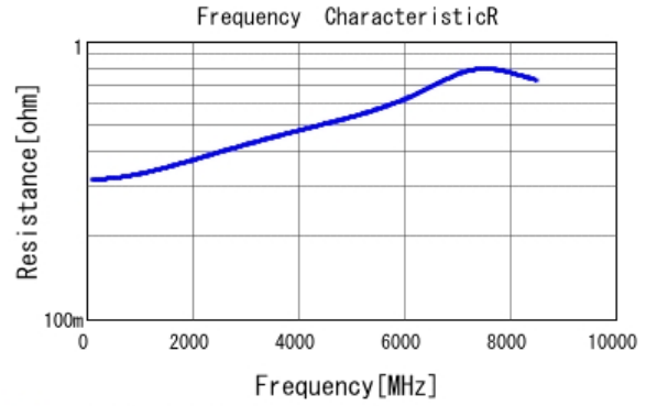
■ GCM1555C1H2R0CA16 R DCOV, 25degC
