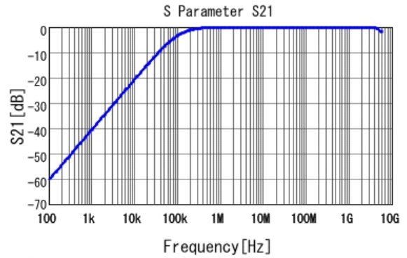
■ GCD188R72A153KA01 S21 DC0V, 25degC
