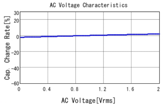
■ GCD188R72A153KA01 C-AC Voltage capchange, DC0V, 25.0d
