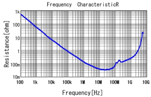
■ GCD188R72A153KA01 R DC0V, 25degC
