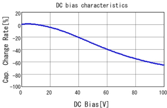
■ GCD188R72A153KA01 C-DC bias capchange, 25.0degC, AC1.
