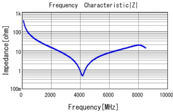
■ GCM1555C1H4R3CA16 |Z| DCOV, 25degC
