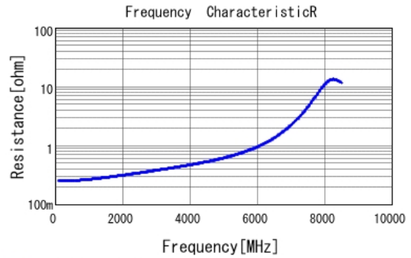
■ GCM1555C1H4R3CA16 R DCOV, 25degC
