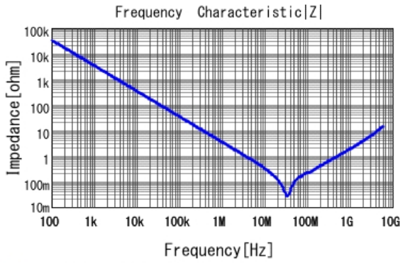
GCM188L81H473KA55 |Z| DCOV, 25degC
