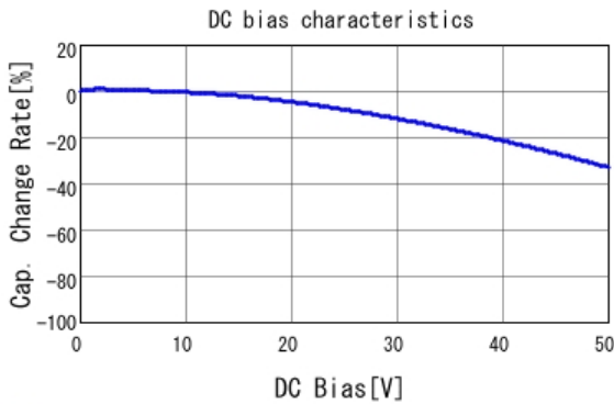
GCM188L81H473KA55 C-DC bias capchange, 25.0degC, AC1.
