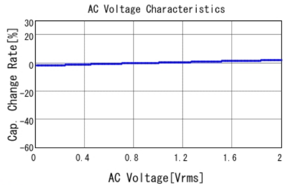
GCM188L81H473KA55 C-AC Voltage capchange, DCOV, 25.0d
