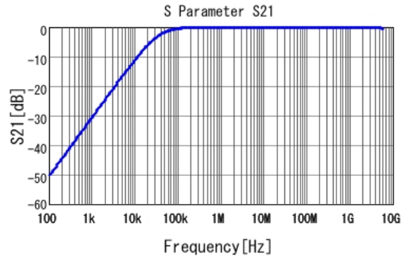
■ GCM188L81H473KA55 S21 DC0V, 25degC
