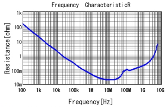
GCM188L81H473KA55 R DCOV, 25degC
