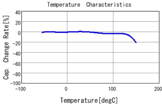
■ GCM188L81H473KA55 C-Temp. capchange, DC0.0V, AC1.0Vrm
