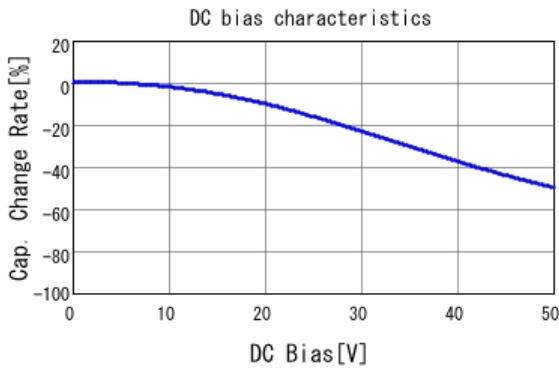
■ GCJ188R71H683KA12 C-DC bias capchange, 25.0degC, AC1.
