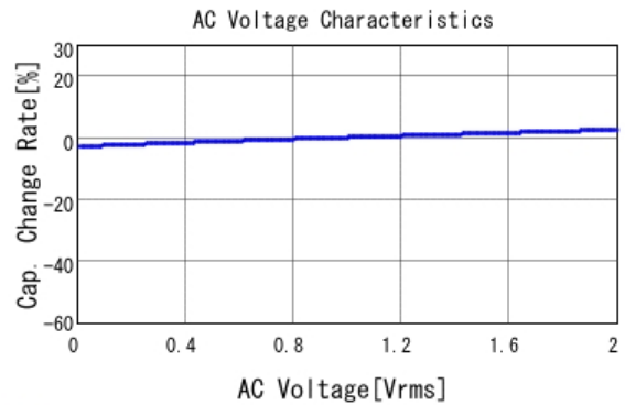
■ GCJ188R71H683KA12 C-AC Voltage capchange, DCOV, 25.0d
