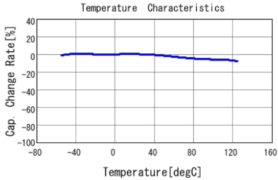
■ GCJ188R71H683KA12 C-Temp. capchange, DC0.0V, AC1.0Vrm
