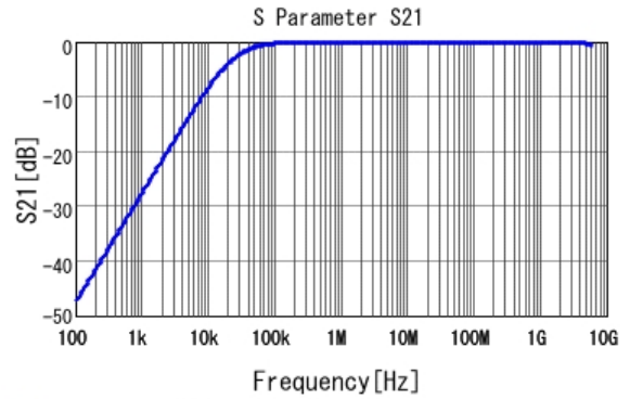
■ GCJ188R71H683KA12 S21 DC0V, 25degC
