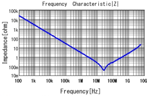
■ GCJ188R71H683KA12 |Z| DCOV, 25degC
