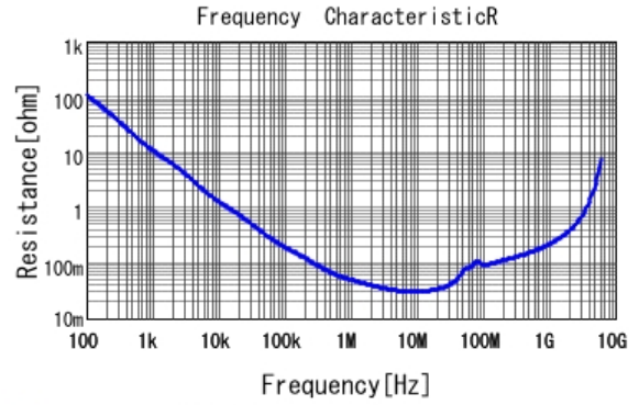
■ GCJ188R71H683KA12 R DCOV, 25degC
