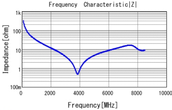
■ GCM1555C1H5R0CA16 |Z| DCOV, 25degC
