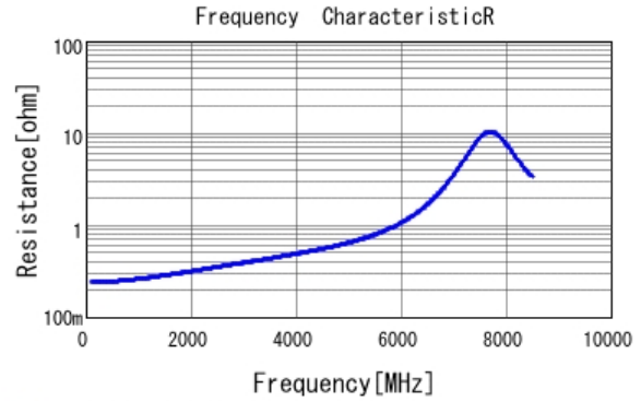
■ GCM1555C1H5R0CA16 R DCOV, 25degC
