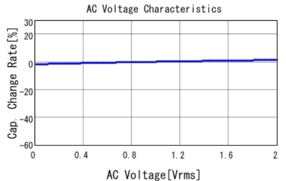
■ GCE188R72A472KA01 C-AC Voltage capchange, DCOV, 25.0d
