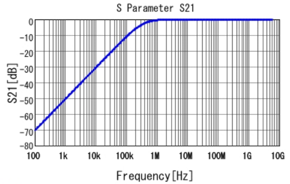
■ GCE188R72A472KA01 S21 DC0V, 25degC
