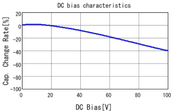
■ GCE188R72A472KA01 C-DC bias capchange, 25.0degC, AC1.
