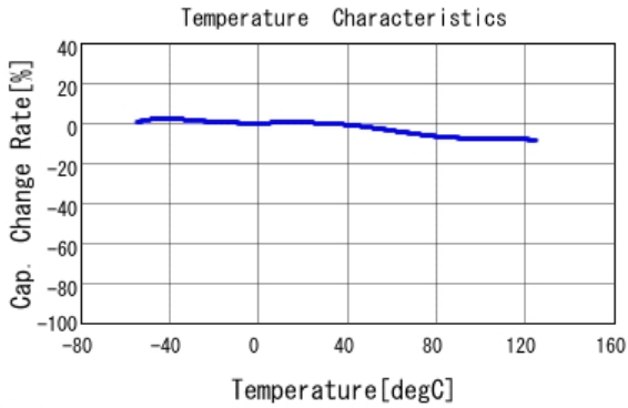
■ GCE188R72A472KA01 C-Temp. capchange, DC0.0V, AC1.0Vrm
