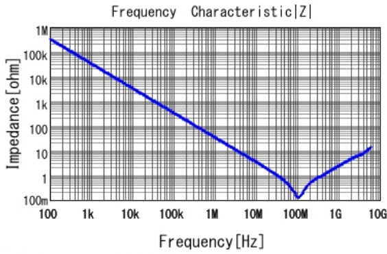
■ GCE188R72A472KA01 |Z| DCOV, 25degC
