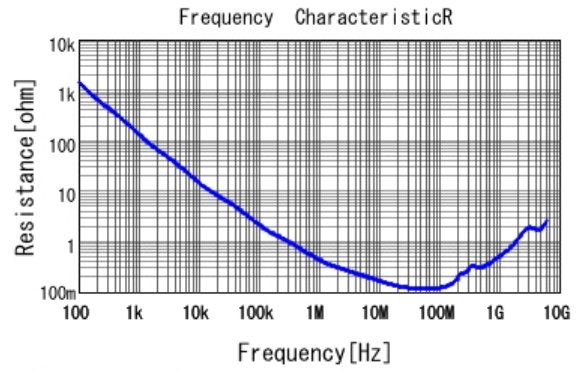
■ GCE188R72A472KA01 R DCOV, 25degC
