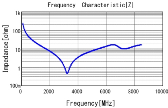
■ GCM1555C1H6R8CA16 |Z| DCOV, 25degC
