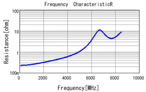
■ GCM1555C1H6R8CA16 R DCOV, 25degC
