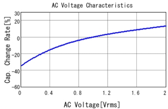
■ GCJ21BR71E225KA01 C-AC Voltage capchange, DC0V, 25.0d
