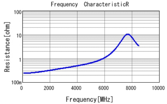
■ GCM1555C1H5R0BA16 R DCOV, 25degC
