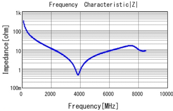
■ GCM1555C1H5R0BA16 |Z| DCOV, 25degC
