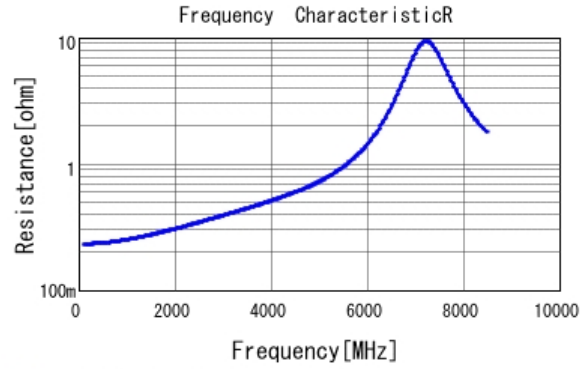
■ GCM1555C1H5R6DA16 R DCOV, 25degC
