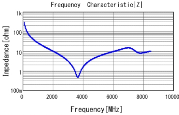
■ GCM1555C1H5R6DA16 |Z| DCOV, 25degC
