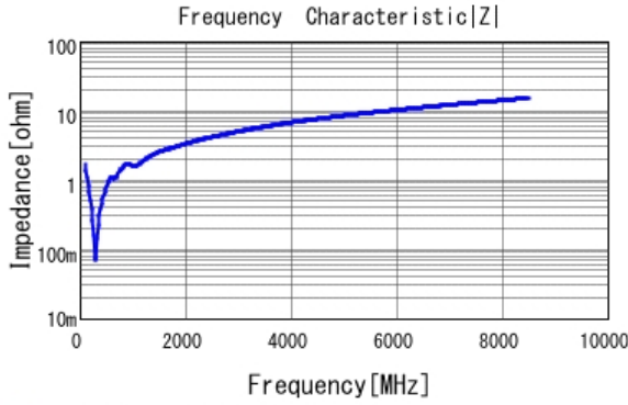
■ GRM1555C1H821GA01 |Z| DCOV, 25degC
