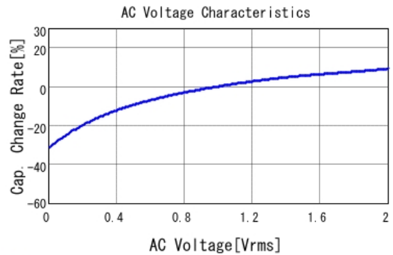
■ GRT21BC81C335KE13 C-AC Voltage capchange, DCOV, 25.0d
