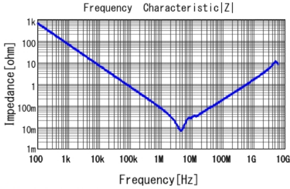
■ GRT21BC81C335KE13 |Z| DCOV, 25degC
