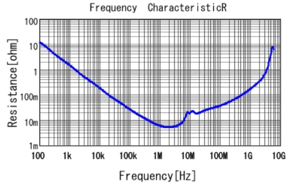
■ GRT21BC81C335KE13 R DCOV, 25degC
