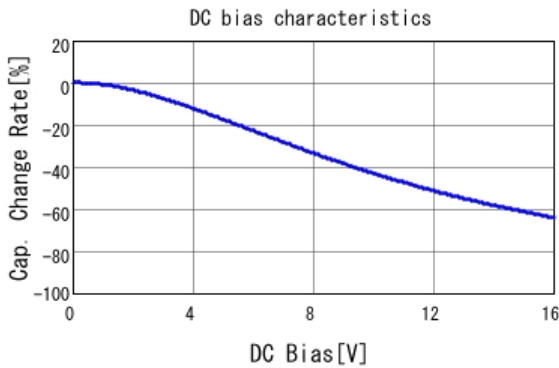
■ GRT21BC81C335KE13 C-DC bias capchange, 25.0degC, AC1.
