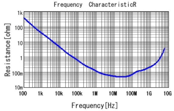
■ GRM155R71C223KA01 R DCOV, 25degC
