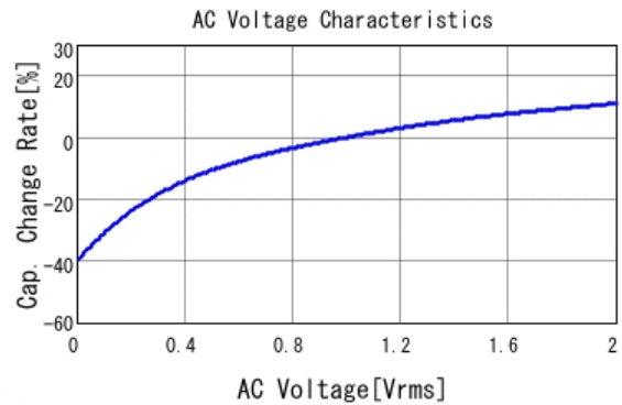
■ GRM155R71A224KE01 C-AC Voltage capchange, DCOV, 25.0d
