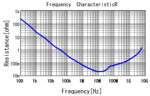
■ GRM155R71A224KE01 R DCOV, 25degC
