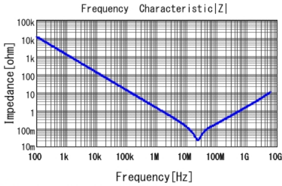
■ GRM155R71A224KE01 |Z| DCOV, 25degC
