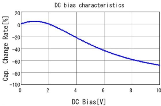
■ GRM155R71A224KE01 C-DC bias capchange, 25.0degC, AC1.
