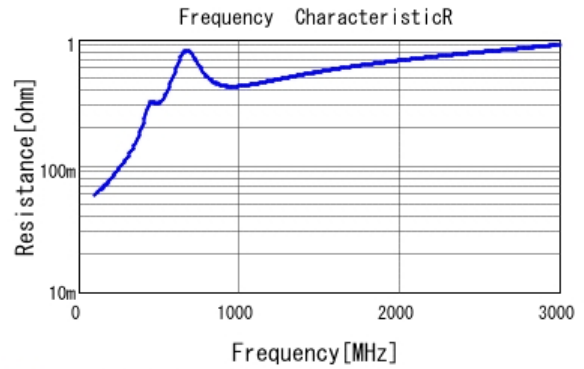
■ GRM21A7U2E821JW31 R DCOV, 25degC
