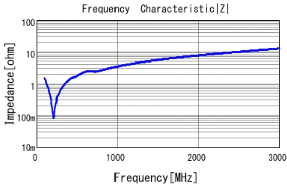
■ GRM21A7U2E821JW31 |Z| DCOV, 25degC
