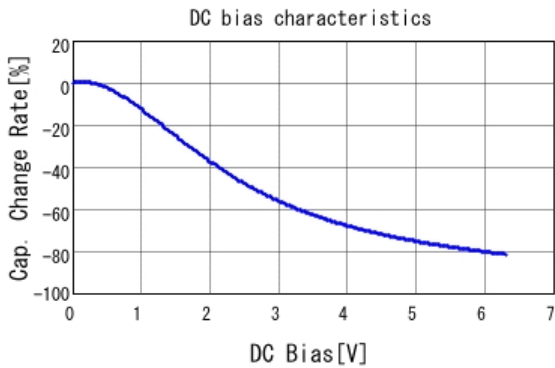
■ GRM187R60J226ME15 C-DC bias capchange, 25.0degC, AC0.
