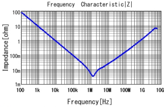
■ GRM187R60J226ME15 |Z| DCOV, 25degC
