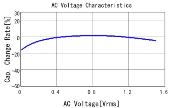
■ GRM187R60J226ME15 C-AC Voltage capchange, DCOV, 25.0d
