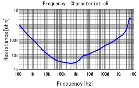
■ GRM187R60J226ME15 R DCOV, 25degC
