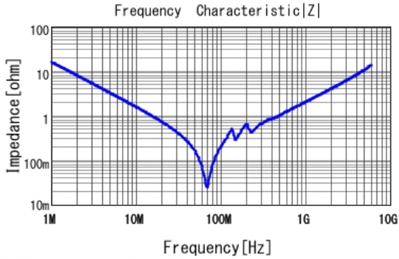
■ GRM2195C1H103JA01 |Z| DCOV, 25degC
