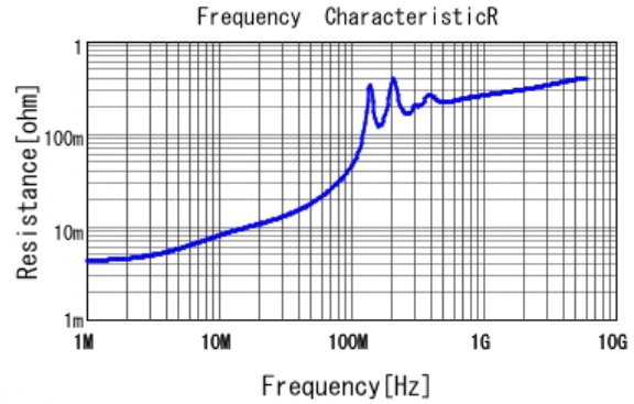
■ GRM2195C1H103JA01 R DCOV, 25degC
