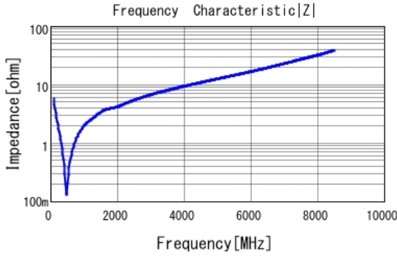
■ GRM1555C1H271GA01 |Z| DCOV, 25degC
