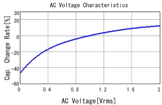
■ GRT155C81C474KE01 C-AC Voltage capchange, DC0V, 25.0d
