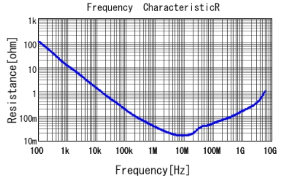
■ GRT155C81C474KE01 R DC0V, 25degC
