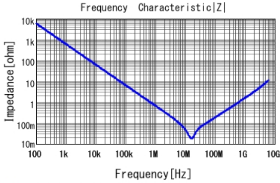
■ GRT155C81C474KE01 |Z| DC0V, 25degC
