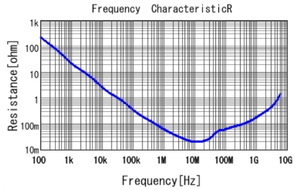
■ GRT155R6YA224KE01 R DC0V, 25degC
