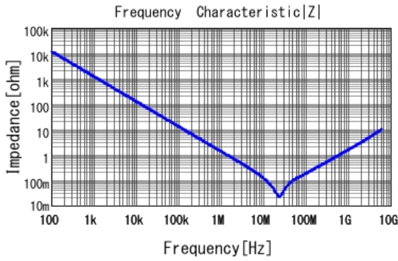
■ GRT155R6YA224KE01 |Z| DC0V, 25degC
