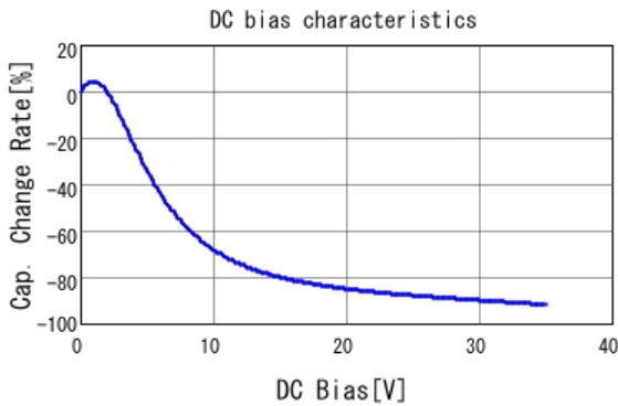
■ GRT155R6YA224KE01 C-DC bias capchange, 25.0degC, AC1.
